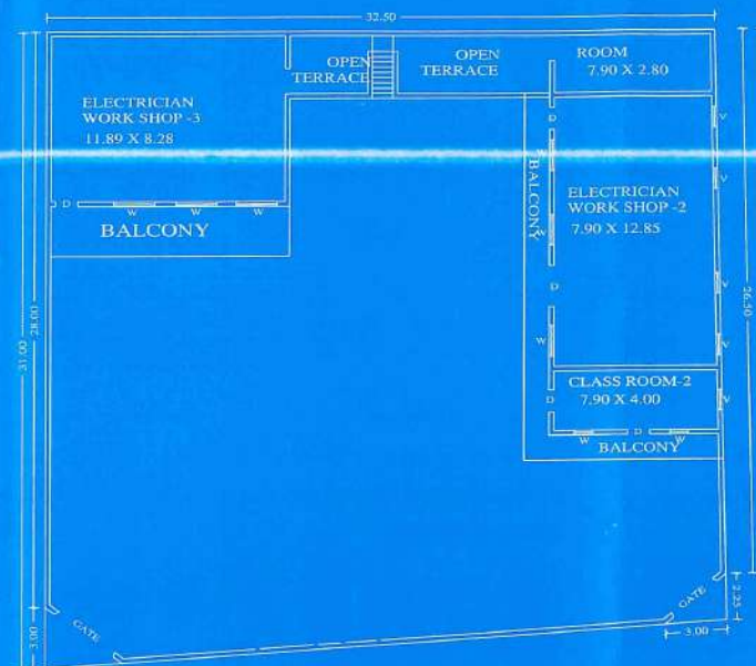
NEW CONSTRUCTION AT FIRST FLOOR
